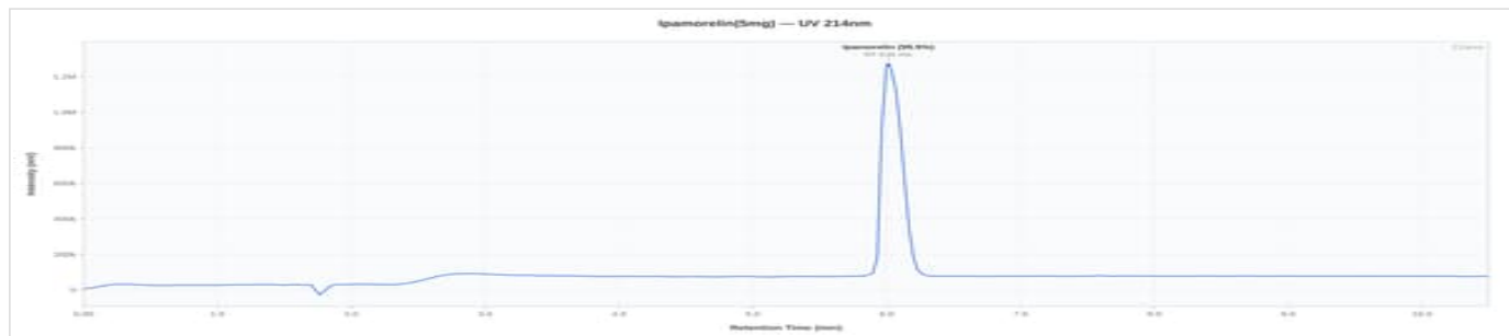
Ipamorelin 5mg - RWBIPA5-1: UV Chromatogram
