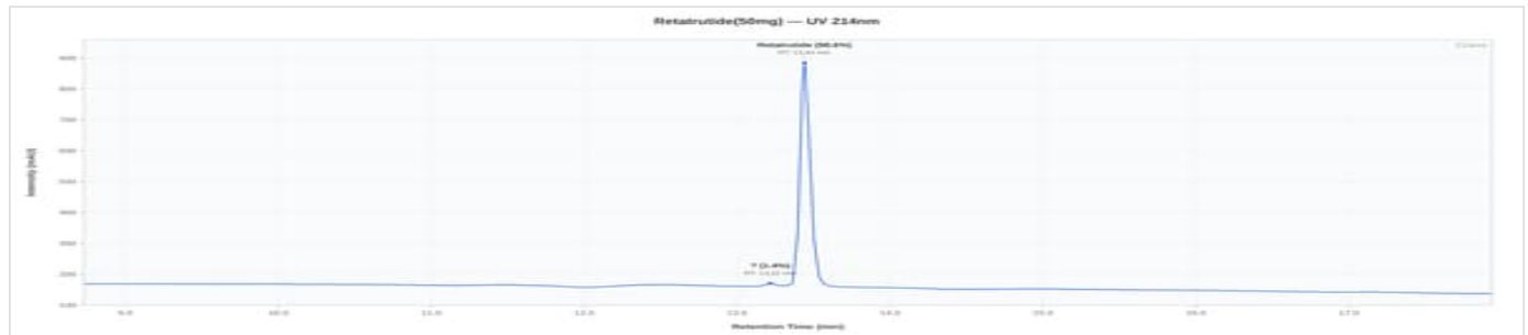
Retatrutide 50mg - RWBRT50-1: UV Chromatogram
