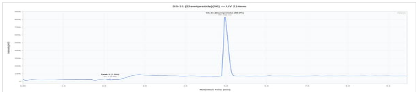
SS-31 50 - RWBSS3150-1: UV Chromatogram
