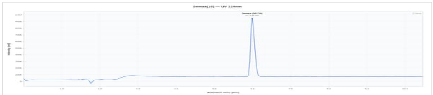
Semax 10 - RWBSMX10-1: UV Chromatogram
