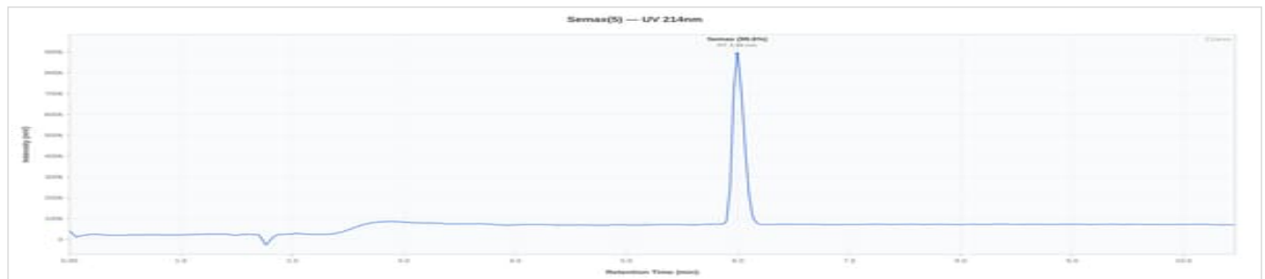
Semax 5 - RWBSMX5-1: UV Chromatogram
